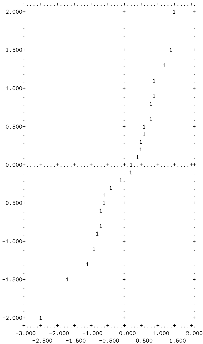
Plot of normal scores (Y) against standardised residuals (X)
